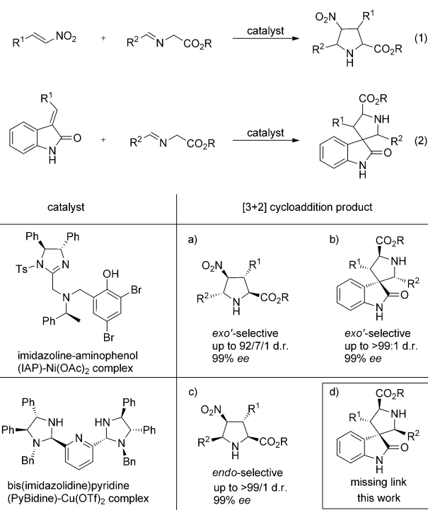
Figure 1. Classification of the stereochemical output of the [3+2] cycloaddition using the IAP–Ni(OAc) 2 catalyst and the PyBidine–Cu(OTf) 2 catalyst.
